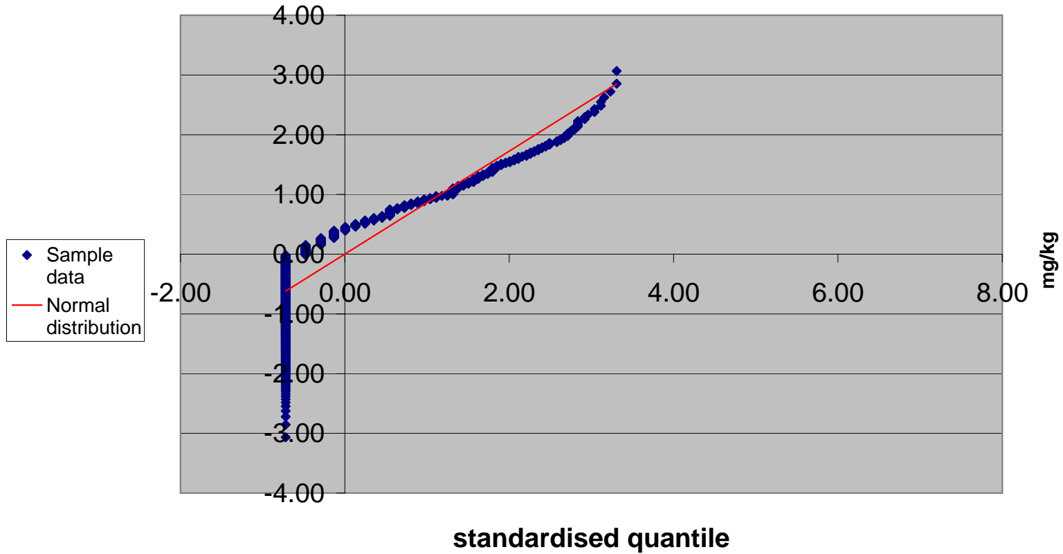
Normal probability plot
