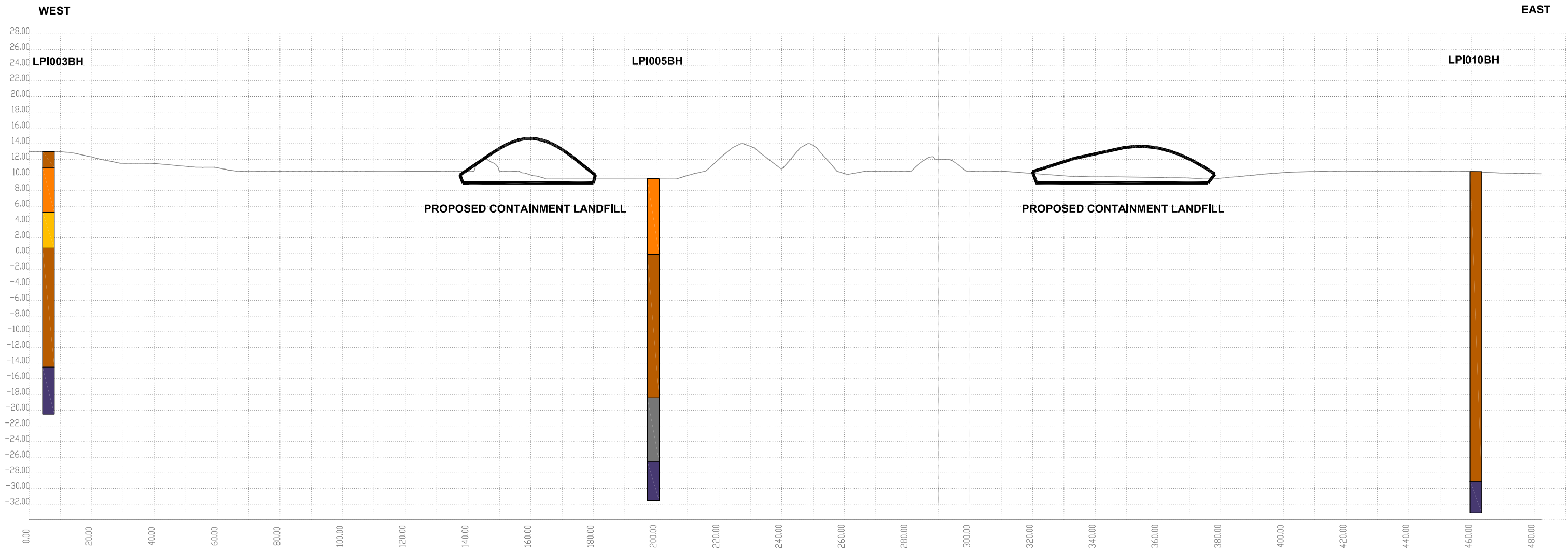
SECTION B-B 1:500 V 1:1250 H
