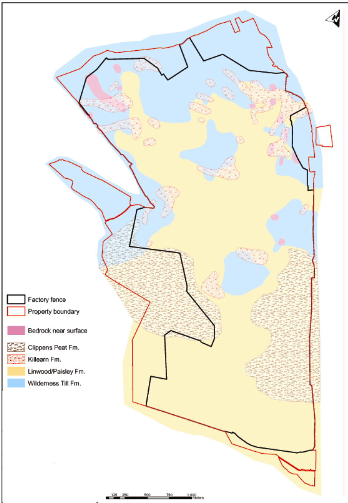
Figure 3 – Refined Superficial Geology Outcrop Plan
