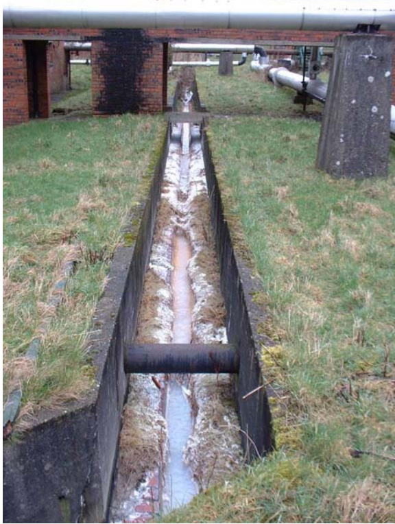
Plate 6.1 - Process drain from 25/105B (Factory I NC Section) showing NC accumulation
